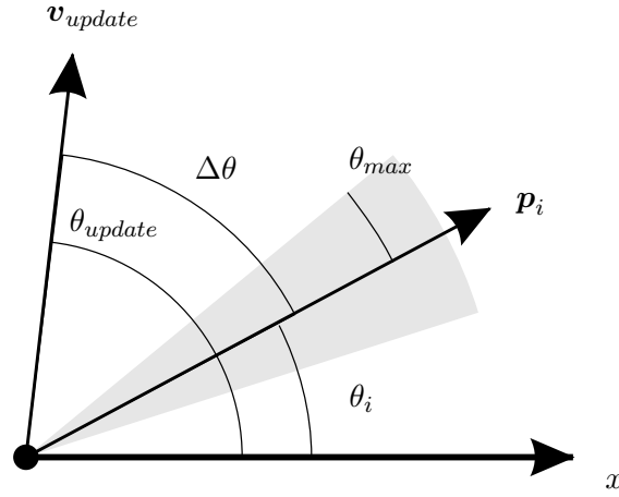
Figure 4.9 Particle Turn Example
